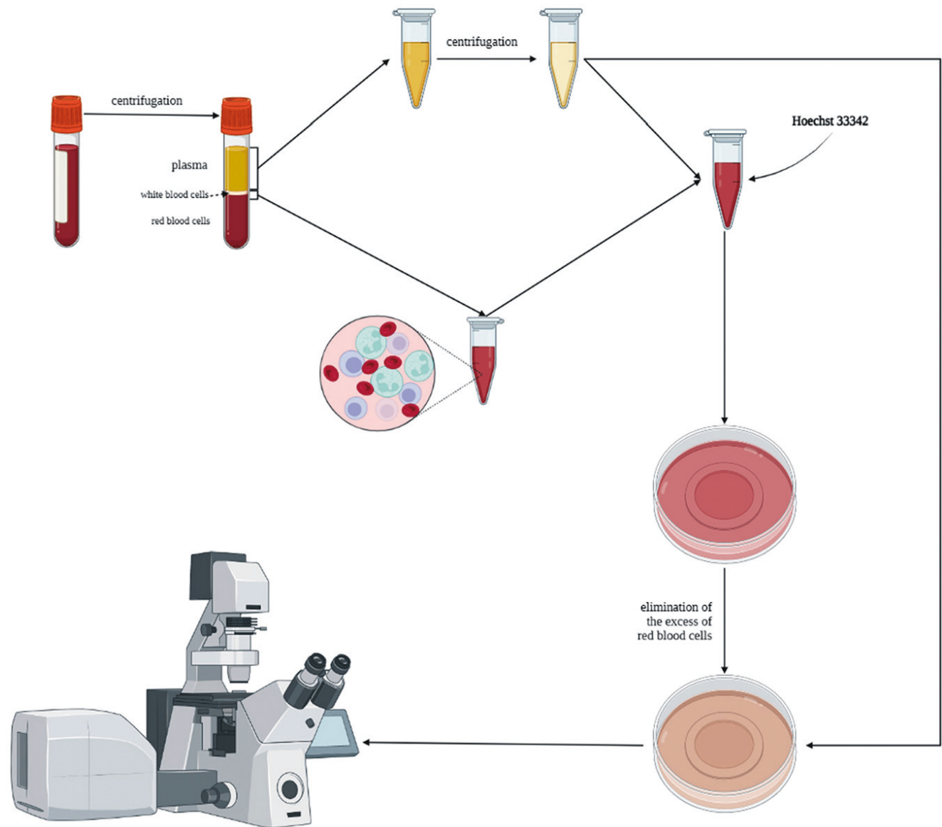
Fig. S1. The scheme of proposed protocol of preparation of samples for studying neutrophils without their isolation.
