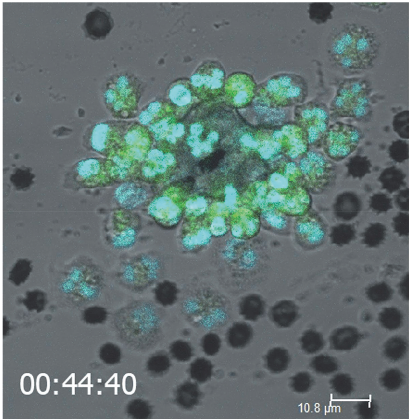
Fig. S2. Neutrophils interact with a foreign particle (larger scale). Blue indicates DNA in neutrophils' nuclei (Hoechst 33342 is used), green indicates HOCl generation (Celestine Blue is used). Black little cells without nuclei are erythrocytes.
